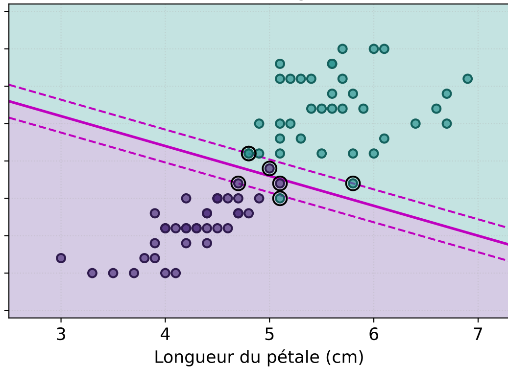
(b) C = 100 : marge = 0.22
