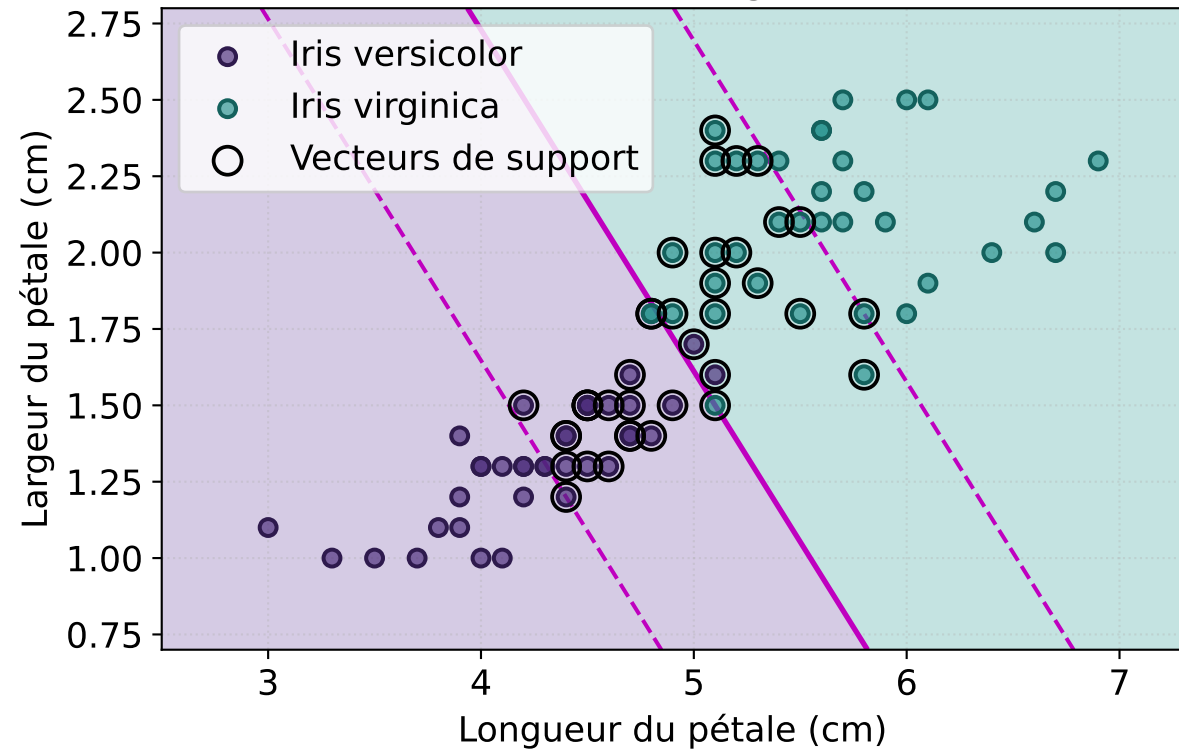
(a) C = 0.1 : marge = 1.44
